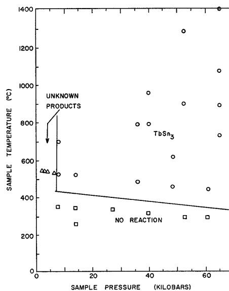
Figure 2.—Tb-3Sn reaction product diagram.
