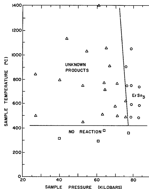
Figure 5.—Er-3Sn reaction product diagram.
