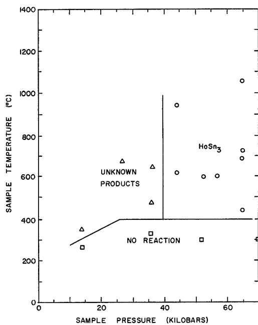
Figure 4.—Ho-3Sn reaction product diagram.
