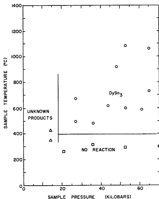
Figure 3.—Dy-3Sn reaction product diagram.
