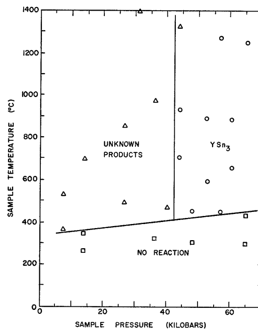
Figure 6.—Y-3Sn reaction product diagram.
